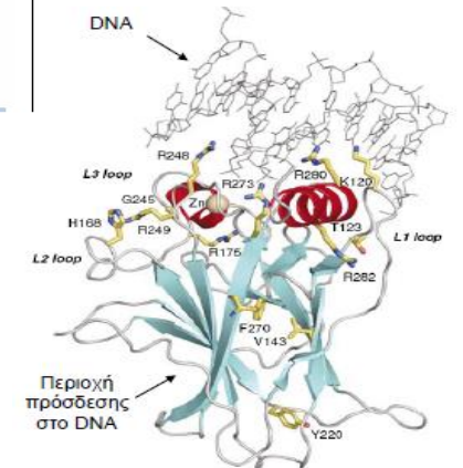
Complex: P53-DNA
